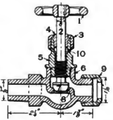
Fig. 3206. 3/8-Inch Globe Valve for Lubricator.
